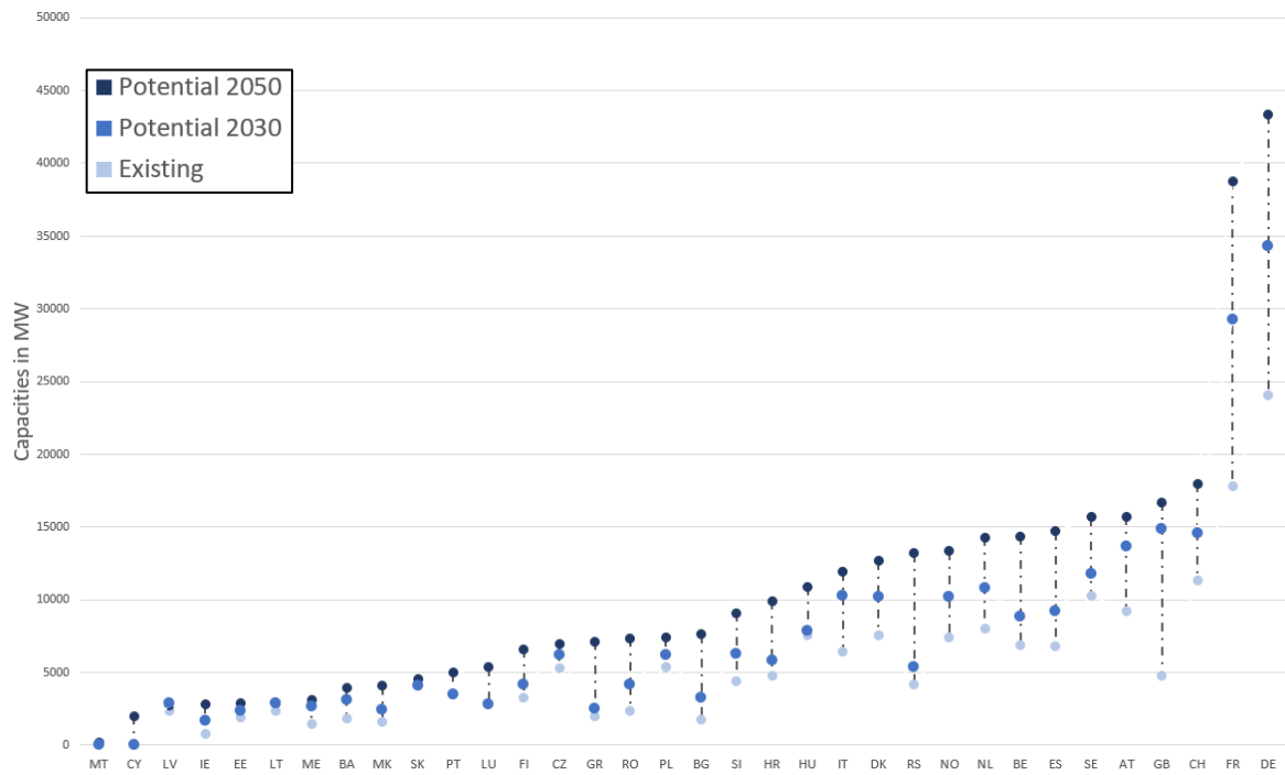
Figure 4 - Interconnectors potential for EU countries
