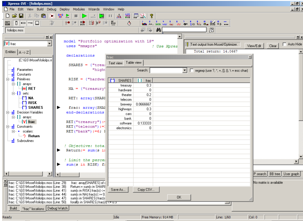
Figure 3.7: Entity display
