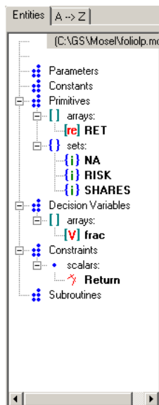
Figure 3.4: Entity display
